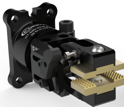
84N2 with Rear Flange Mount and Double Blank Detector Sensor Kit
